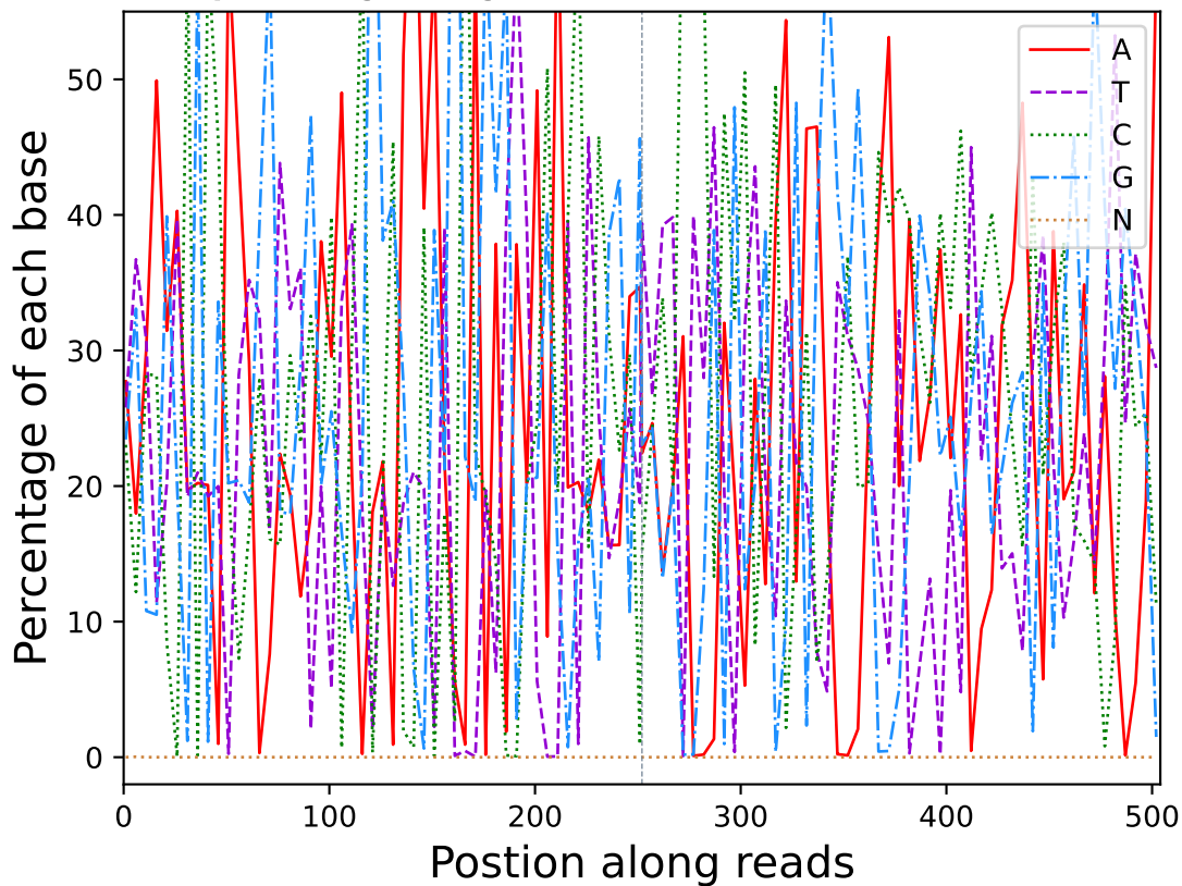
Base percentage along reads (R20109)
